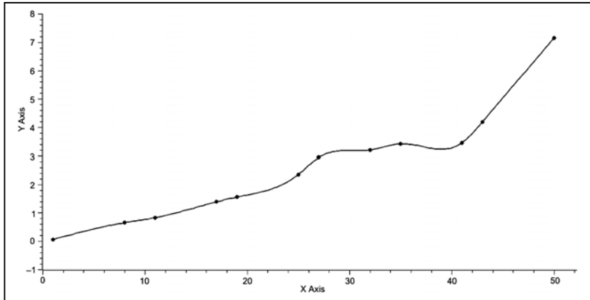
Fig. 10. Time is represented on the x-axis, and the magnitude of the maxima of both X = S\cos\Psi and Y = S\sin\Psi is represented on the y-axis. The periodicity of the maxima of both X and Y is apparent. This graph was created with the use of spline interpolation
